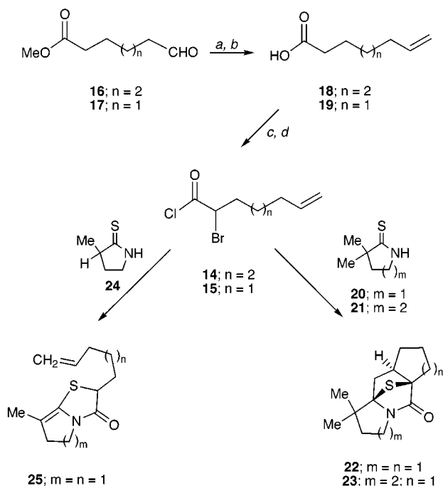
Scheme 4 a
