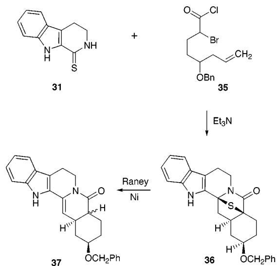
Scheme 8
