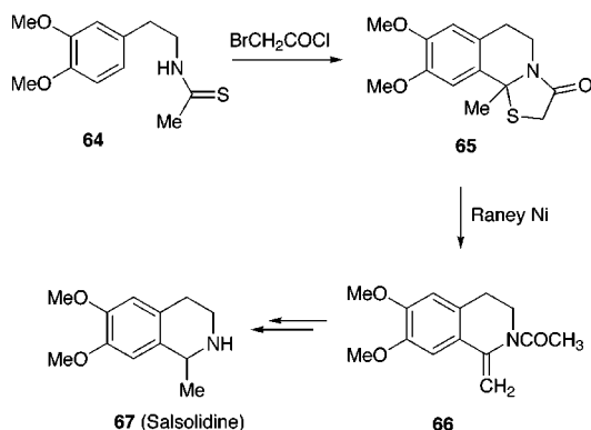
Scheme 13
