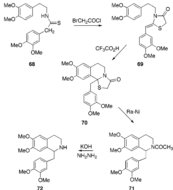
Scheme 14
