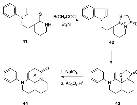
Scheme 9
